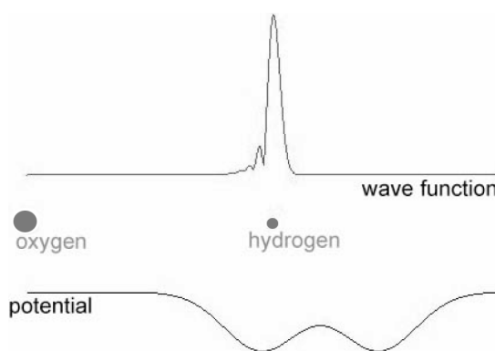
Figure 6 Two water molecules become closer; the wave function has broken into pieces and the vibration of the wave function of the hydrogen atom has ceased
